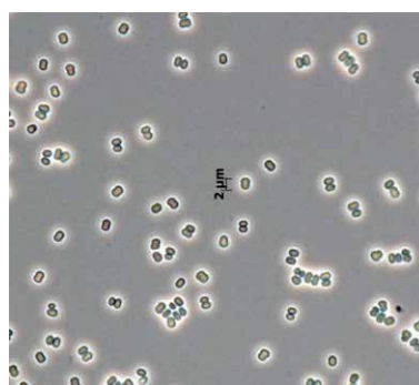
Staphylococcus hominis
