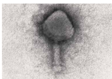
Bixzunavirus dandelion
